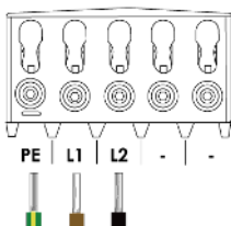
IT/TT 1-phase (230V)
