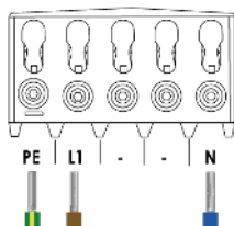
TN 1-phase (230V)
