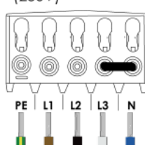
IT/TT 3-phase (230V)
