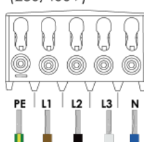
TN/TT 3-phase (230/400V)
